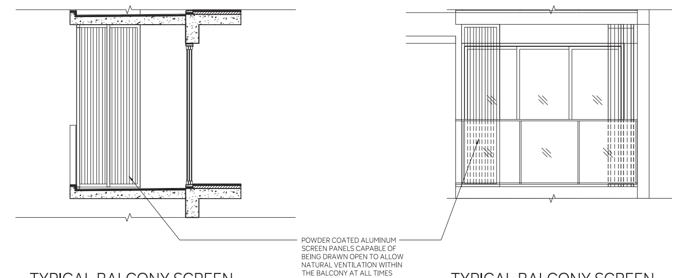
TYPICAL BALCONY SCREEN (CLOSED)
